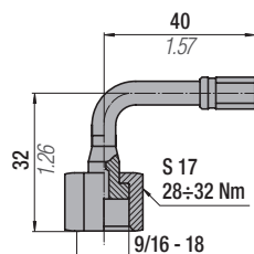
code 36P9/1602
