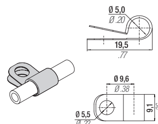
code: 36FF06A
