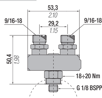
code PA-M6
